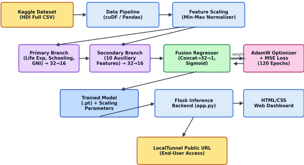
Figure: End-to-end solution architecture, from Kaggle dataset ingestion to the deployed web dashboard.
